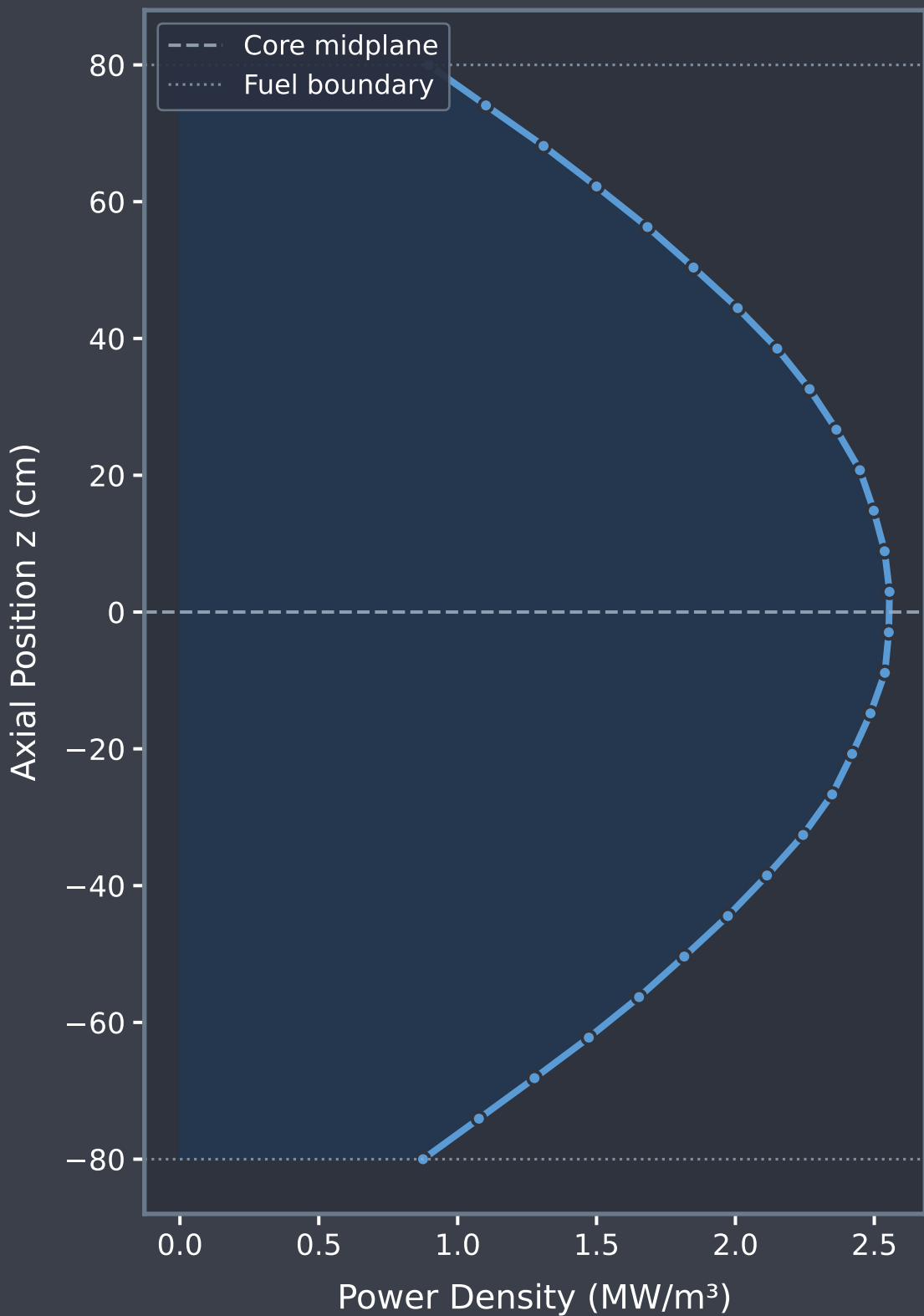
TRAVIS Core — Axial Power Distribution (normalized to 2.5 MWth)
